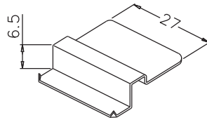
[中棧止金具] 135-H
