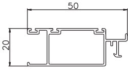
[召合せ材] 194-H
