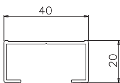
[横材] 201-H
