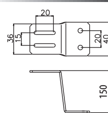
[足長金具] 214-H
