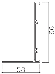
[縦材] 407-H
